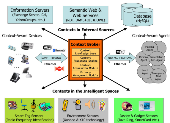
Figure 1: A context broker acquires contextual information from heterogeneous sources and fuses it into a coherent model that is then shared with computing entities in the space.
