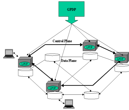
Fig. 2. Overlay Network
