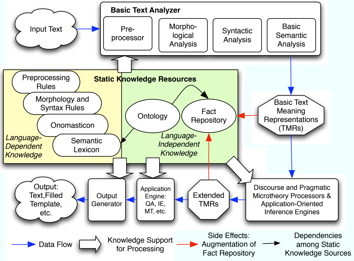
Fig. 1. OntoSem is a large scale, sophisticated natural language understanding system that uses a custom frame-based knowledge representation system with an extensive ontology and lexicon.
