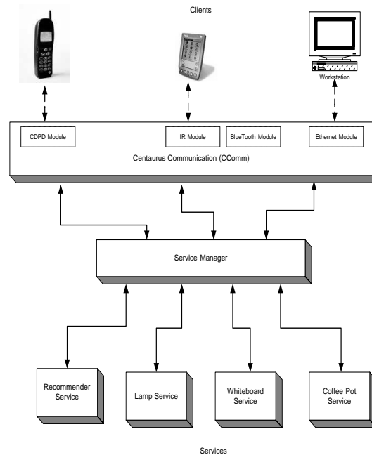
Fig. 1. Centaurus Components
